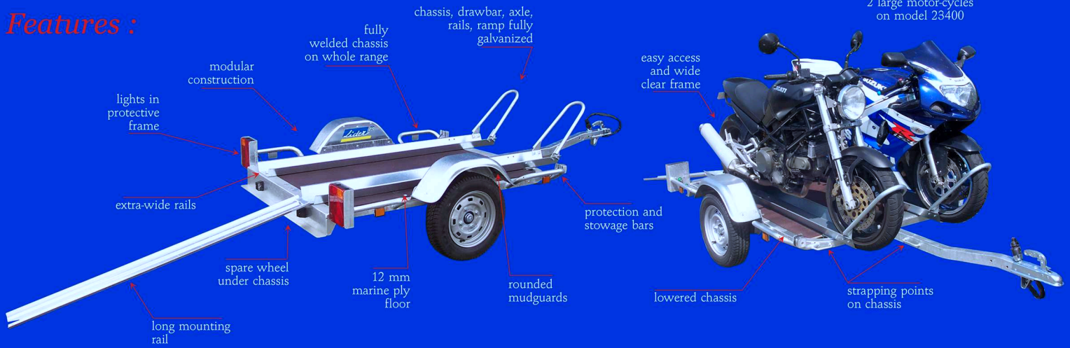
Model shown : 23401 fitted with 2 rails, 1 ramp and non slip floor
